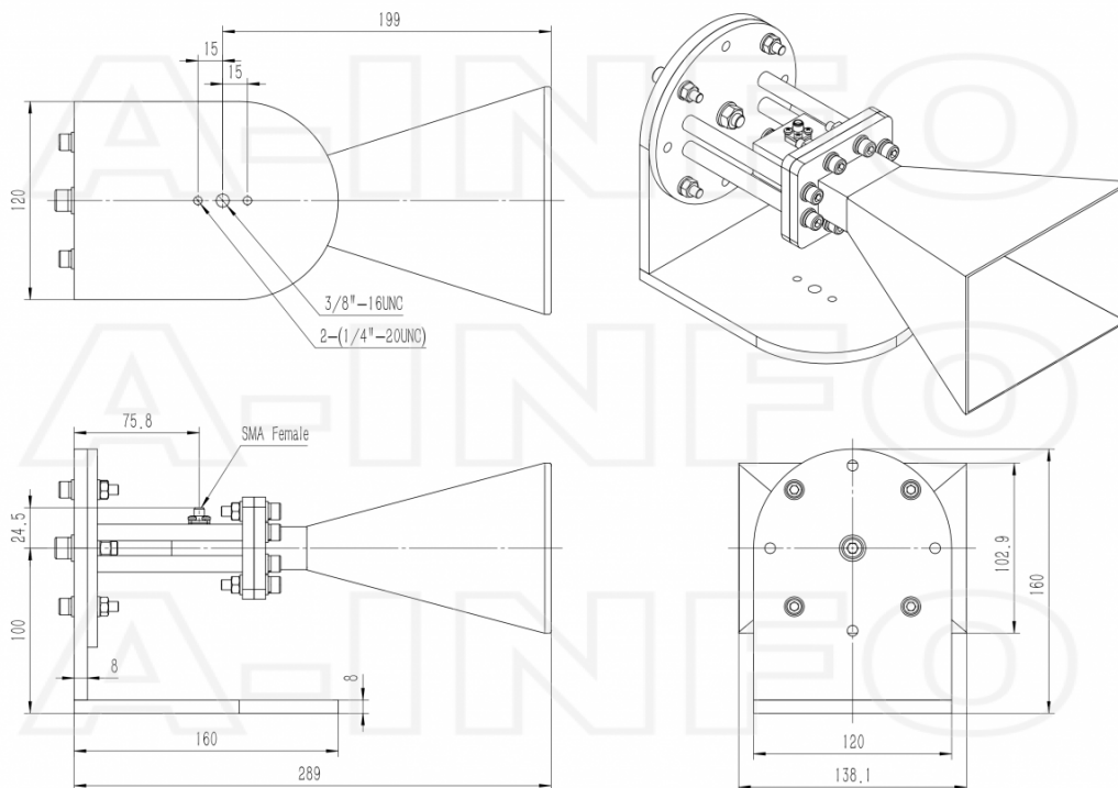
SMA Female Output with L Type Mounting Bracket (Option, P/N: LB-159-10-C-MBL)
