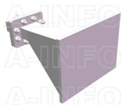
LB-159-15-C-3.5FSPO Standard Gain Horn Antenna 4.9-7.05GHz 15dB Gain 3.5mm Female
